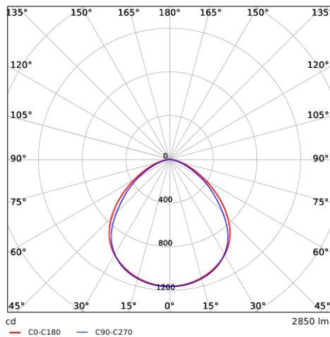
LEDFlood-E2 Re199-30W-3000-BL
