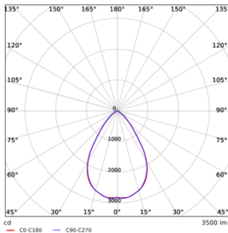
LEDDownlightRc-P-HG R200-33W
