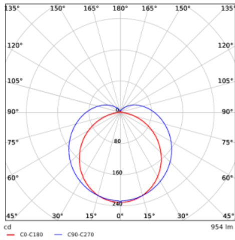
LED E T5 batten 900
